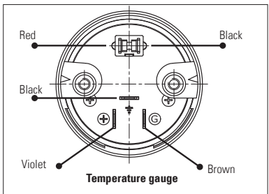
Connections of the temperature gauge
