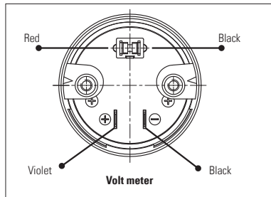
Connections of the volt meter
