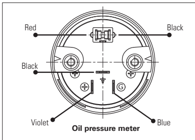
Connections of the oil pressure gauge
