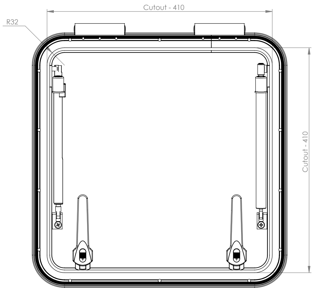
Dimension Including Mosquito Screen
