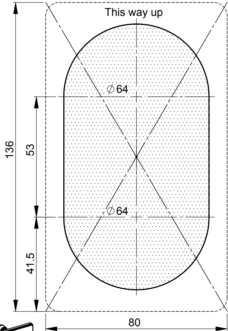
Drill pattern for: Alfa 30T
