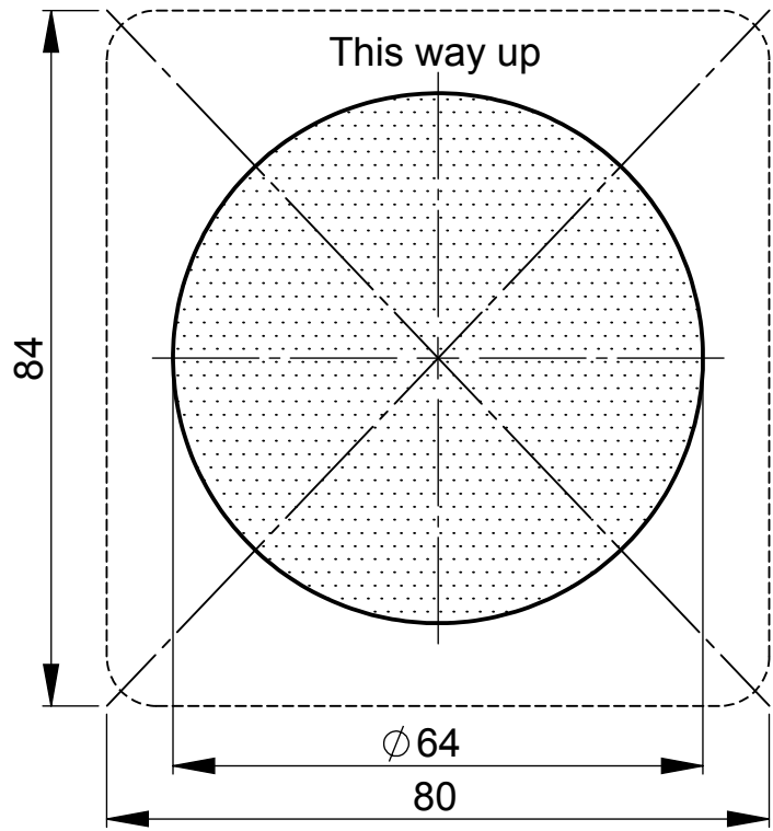
Drill pattern for: Alfa 10T - Alfa 20T
